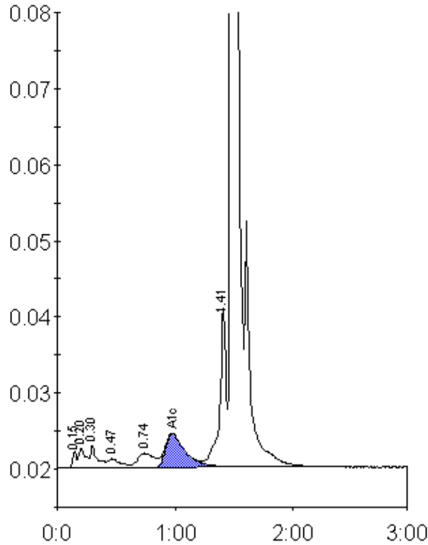
Peak table - ID: 10571198
